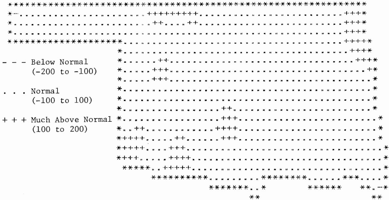
FEBRUARY 1988 DEVIATION FROM NORMAL HEATING DEGREE DAYS
